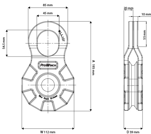
Pulley Housing
